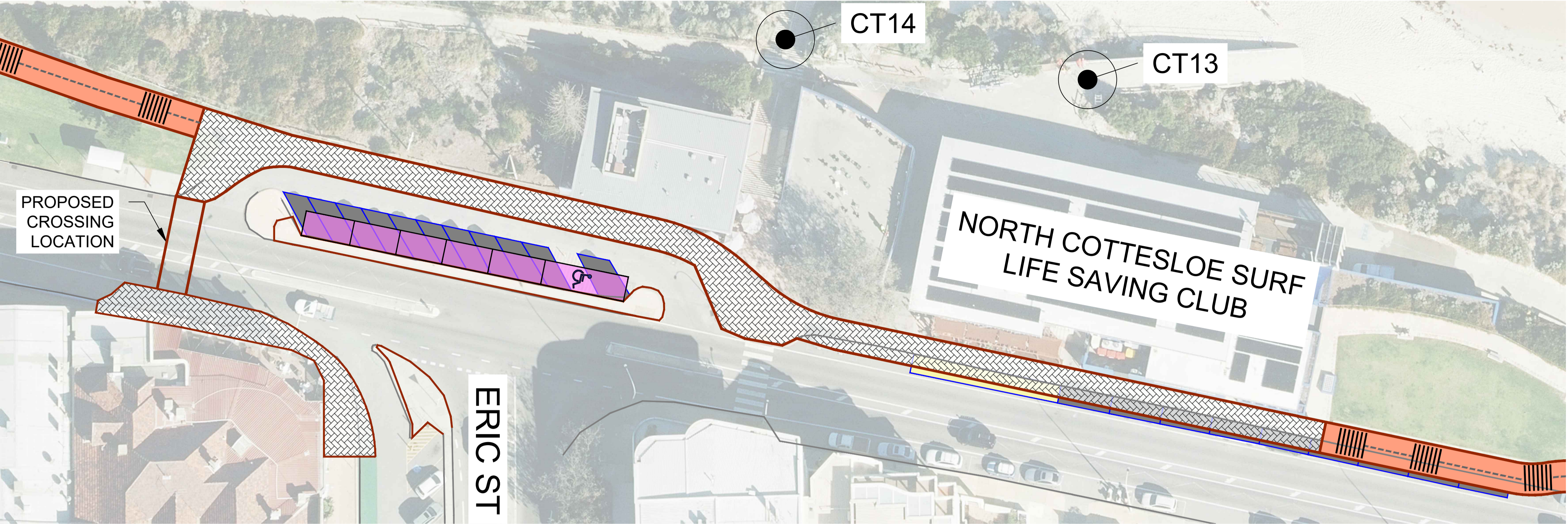
CONFLICT LOCATION 3 - OPTION 1: NORTH COTTESLOE SURF LIFE SAVING CLUB (SHARED ZONE)
