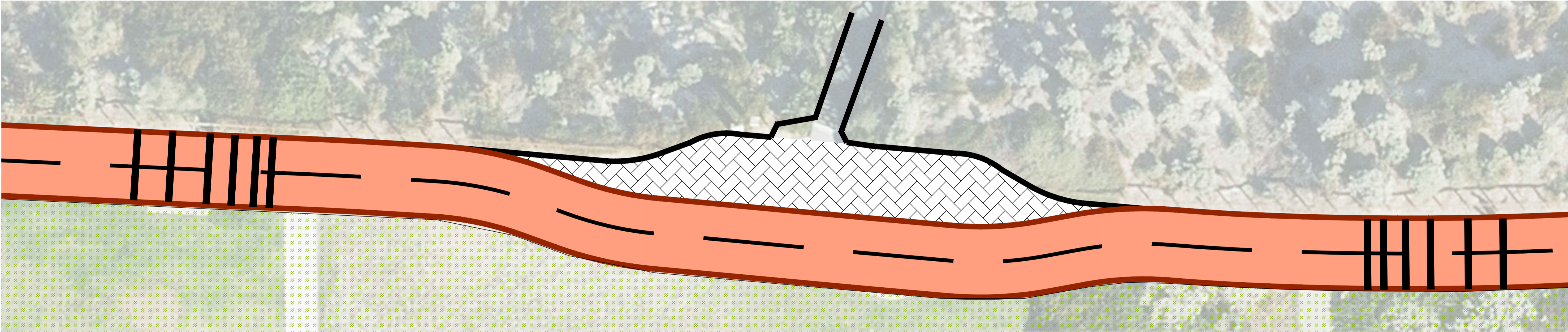
CONFLICT LOCATION 1 - OPTION 2: BEACH ACCESS PATH ENTRY POINTS (TYPICAL DIAGRAM)
